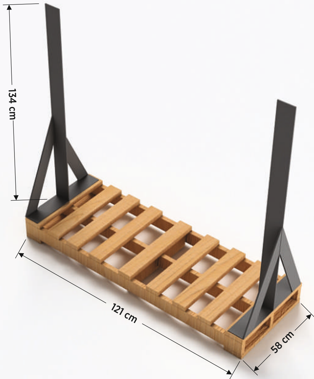
20 BOX PALLET For 1200x1200mm Tiles
